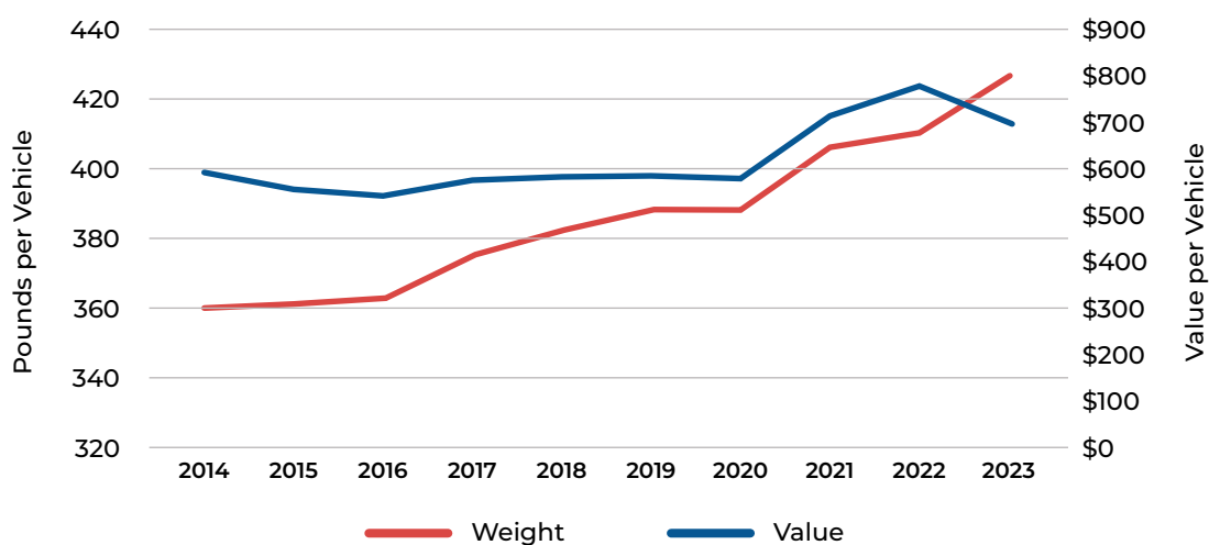
Figure 5. Plastics per Vehicle—Weight vs. Value
