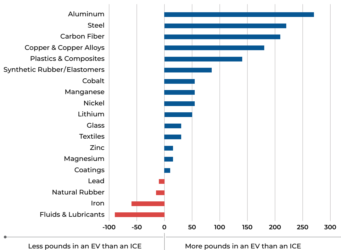
Figure 7. Material Composition—Difference Between EV and ICE Vehicles
